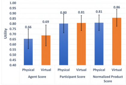
Figure 5: Avg. individual utilities and normalized product scores
