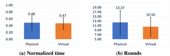
Figure 6: Average agreement time and negotiation round
