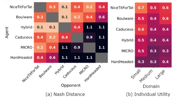
Figure 4: Opponent-Based (a) & Domain-Based (b) Analysis
